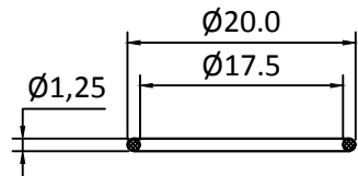
“O”RING
