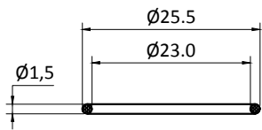
“O”RING
