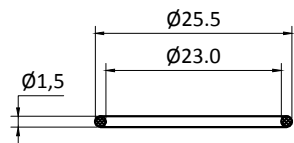
“O”RING
