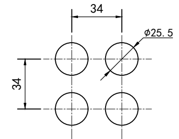
Install size
