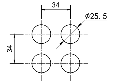
Install size
