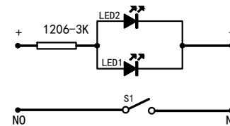
Switching Circuit
