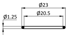
“O”RING
