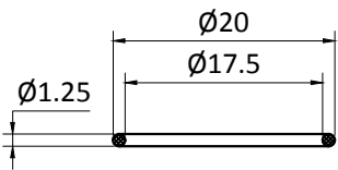
"O"RING
