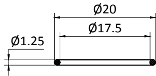
“O”RING
