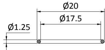
“O”RING
