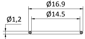
“O”RING
