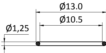
“O”RING
